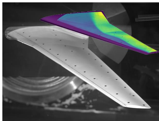
Fig 1: Pressure sensitive paint measurements on a wing performed in the ONERA S3Ch transonic wind tunnel, clearly showing the transonic buffet phenomenon.
